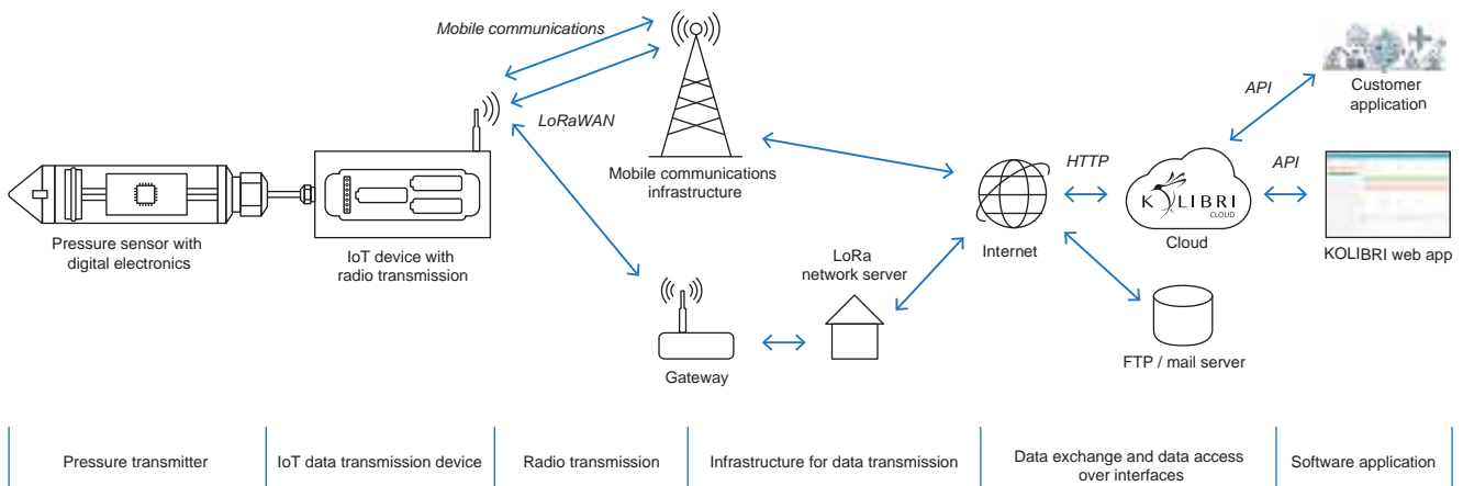
Remote transmission with LoRaWAN or NB-IoT networks
