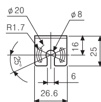
●Bracket A
