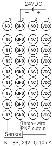
ARD-DI08P-4S
