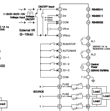
DPU3 Series(3 Phase)
