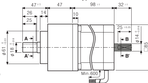
<Geared type>
