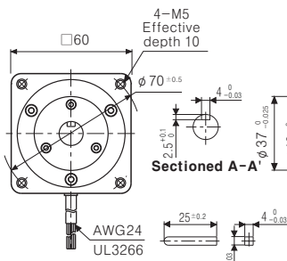
Parallel Key
