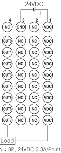
ARD-DO08N-4S
