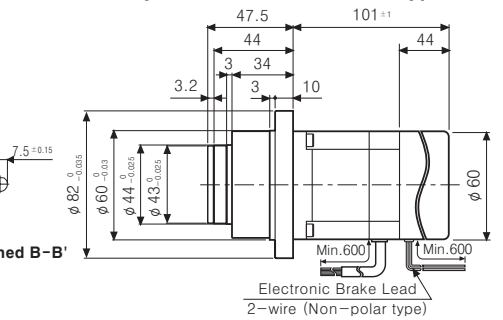
<Rotary actuator+Brake built-in type>
