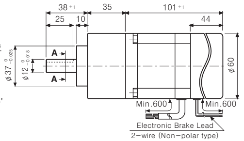
<Geared+Brake built-in type>
