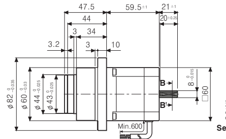
<Rotary actuator type>
