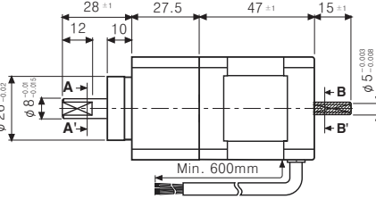
<Geared built-in type>
