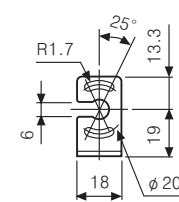
●Bracket B
