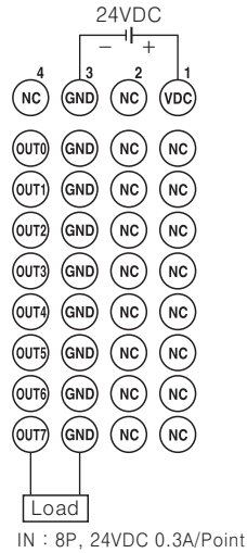
ARD-DO08P-4S
